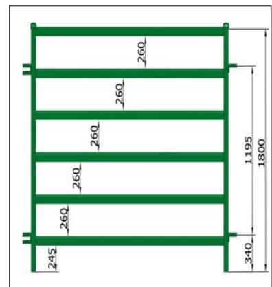
Oval pipe's typical pitch
